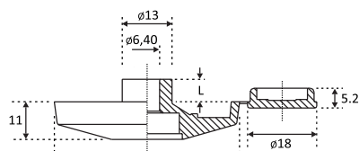
Polyamide (Nylon) large washer
