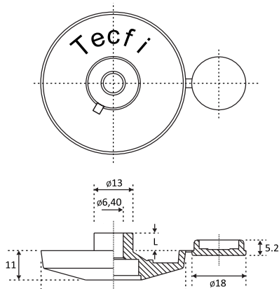
Rondella larga in poliammide (Nylon)
